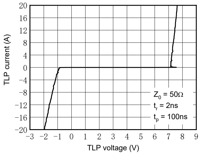
Fig.9 TLP Measurement
