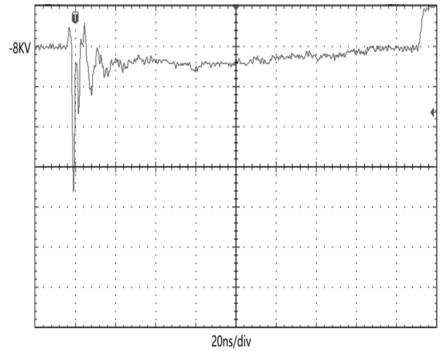
Fig.8 ESD clamping (-8kV contact discharge per IEC61000-4-2)
