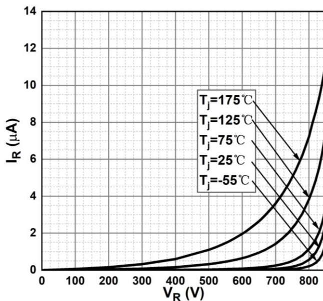
Figure 2. Reverse Characteristic
